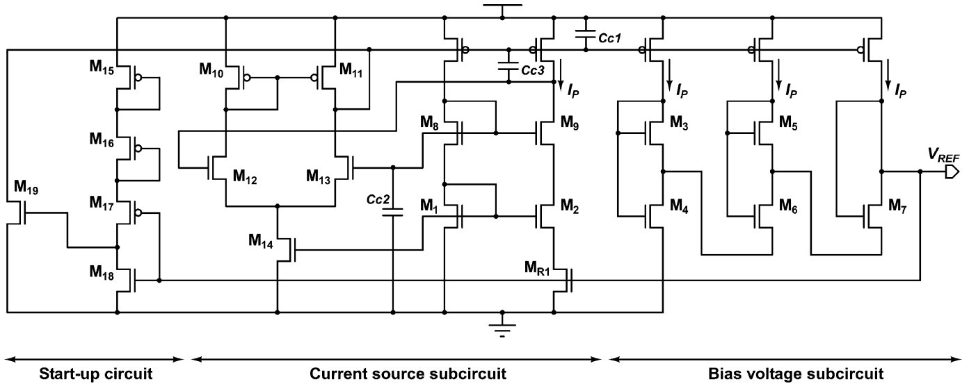
Fig. 3. Entire circuit of our voltage reference. All MOSFETs are operated in subthreshold region, except for MOS resistor M_{R1} , which is operated in strong-inversion, triode region.
