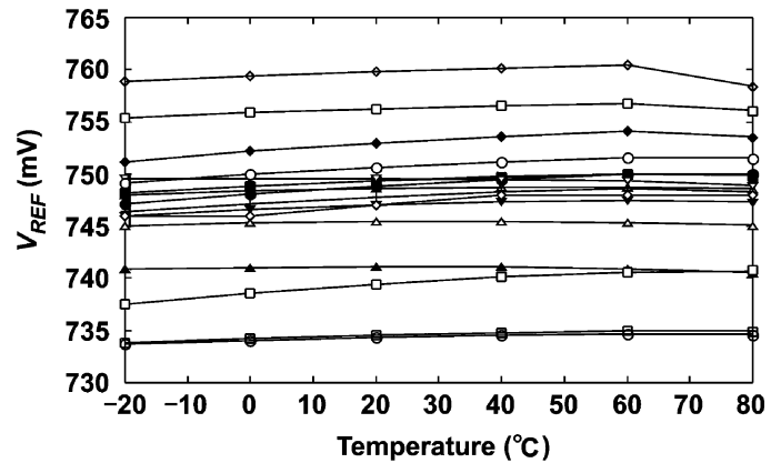
Fig. 11. Measured output voltage V_{REF} as a function of temperature for 17 samples on different chips from same wafer. Supply voltage was set to 1.5 V. Temperature coefficients from 7 to 45 ppm/ ^{\circ} C were observed. Average TC was 15 ppm/ ^{\circ} C.
